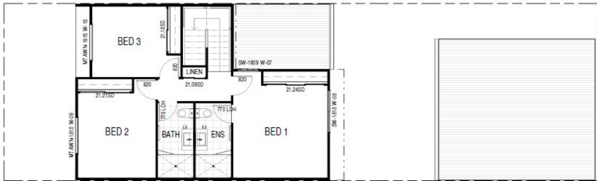
1 FIRST FLOOR PLAN 1:100
